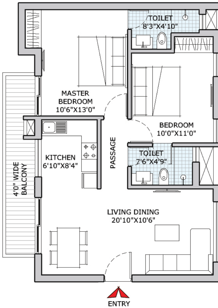
TYPICAL UNIT PLAN
