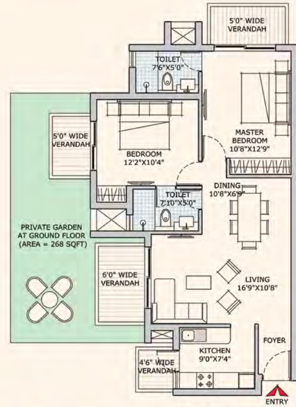
UNIT PLAN
